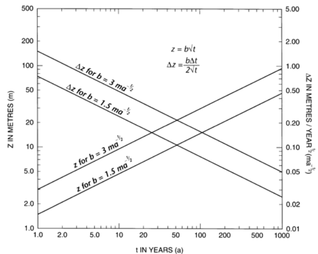
FIGURE 3. Nomogram for the growth of permafrost (z) and rate of growth (Δz) given two typical freezing conditions for the Tuktoyaktuk Peninsula Area. See text.
