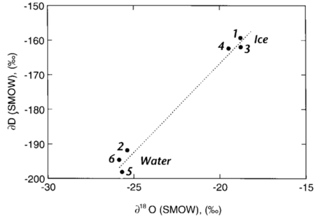
FIGURE 49. Co-isotope plot of \delta^{18}\text{O} (SMOW) and \delta\text{D} for the sample sites given in Figure 48 and Table V. The co-isotope slope is about 5.2.
