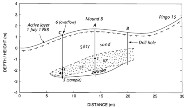
FIGURE 48. Vertical profile of Frost Mound B (see Fig. 46 for the location of the profile). The numbers refer to sample sites for water quality analyses as given in Table V.
