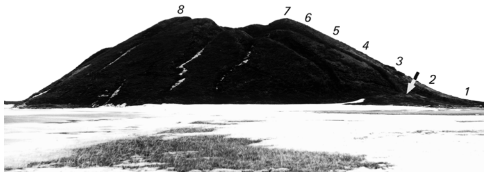
FIGURE 56. Pingo 18 (Ibyuk Pingo) showing the locations of BM 1 to 8. The arrow marks a slump formed by wave undercutting during a rise in sea level that accompanied a storm surge.
