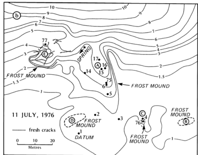
FIGURE 53. a) A map of the "area of spring flow" (Fig. 40) of Pingo 17 for August 1975. b) Map of the same area as in Figure 53a but for July 1976. See text for a discussion of the changes in the individual frost mounds and for the new frost mound at E.
