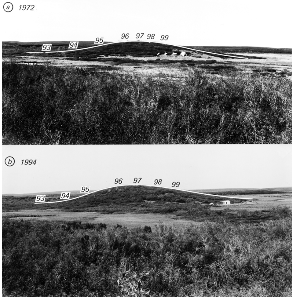
FIGURE 15. a) 1972 photograph of Pingo 7 (Porsild Pingo). Datum BM 92 is off the left side of the photograph. BM 93 to 99 are on the pingo. b) 1994 photograph taken from essentially the same site as the 1972 photograph. A comparison of the 1972 and 1994 photographs shows a combination of both pingo and willow growth. See text.
