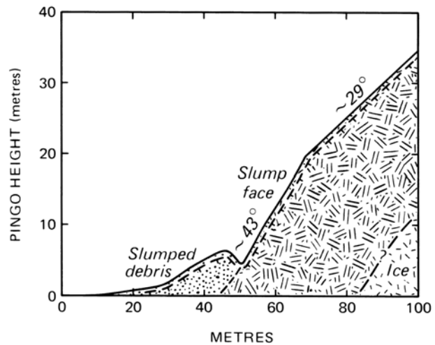
FIGURE 60. Cross section of the slump shown by the arrow in Figure 56. The slump was caused by wave erosion when there was a rise of sea level that accompanied a severe storm surge. The failure surface was in permafrost.
